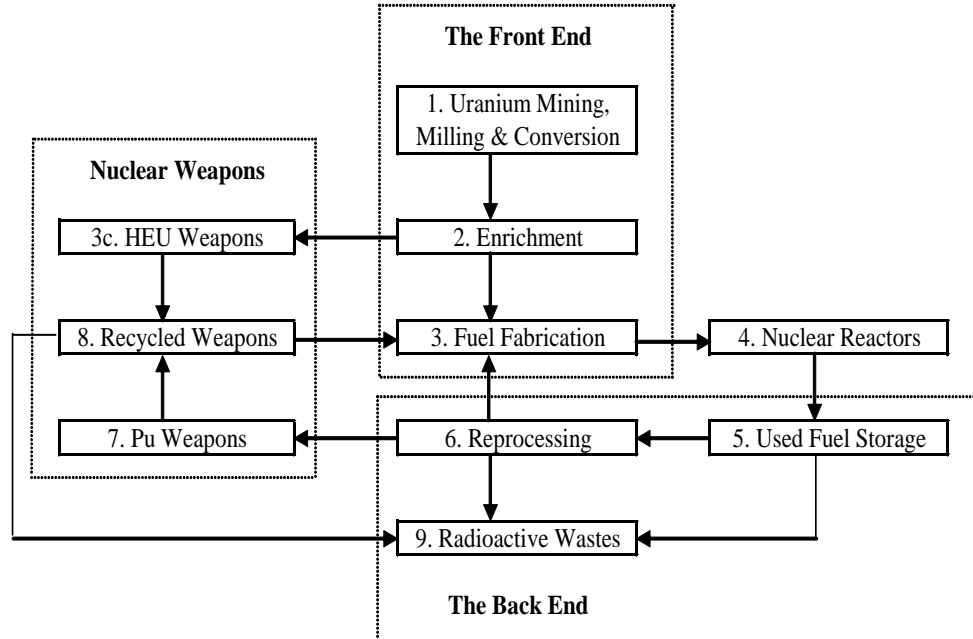
Figure 3: The Light Water Reactor Nuclear Fuel Cycle
